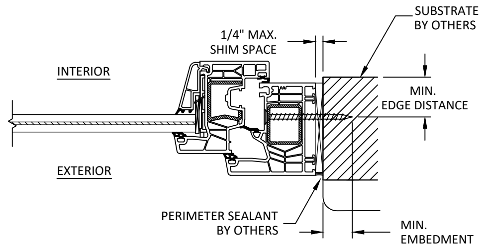
ANCHOR DETAIL THROUGH FRAME (JAMB)
