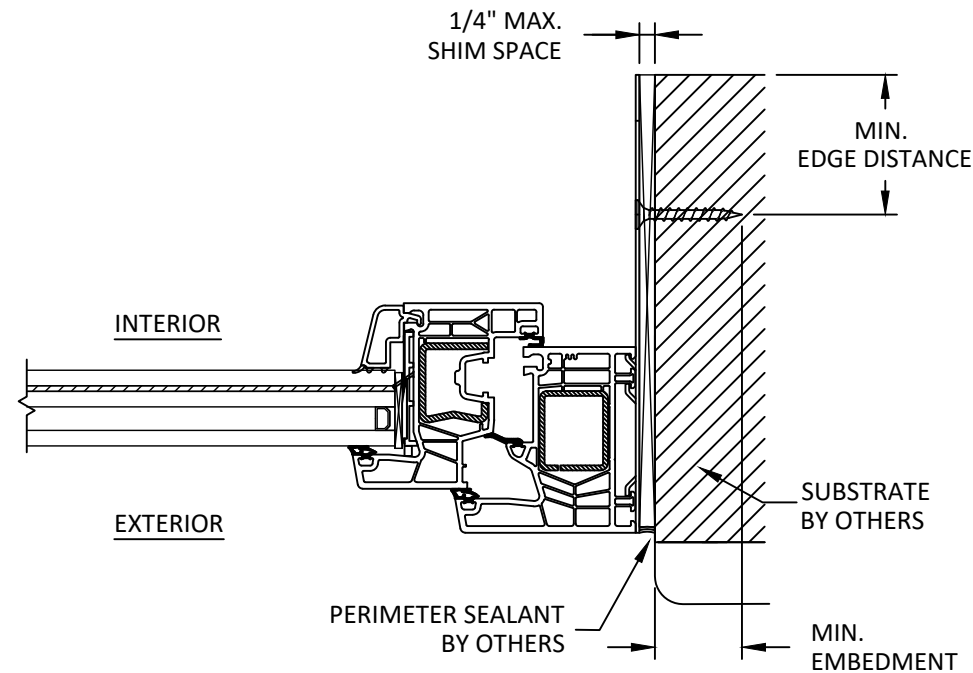
ANCHOR DETAIL STRAP (JAMB)
